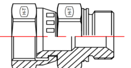
FJS-MM Straight
