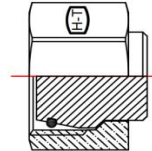
METRIC LIGHT SERIES TUBE CAP
