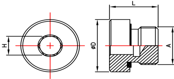
MBSPP-Hollow Hex Plug
