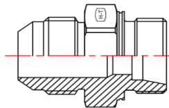
MJ-MM Dual Purpose (S)
