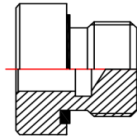
MM Hollow Hex Plug
