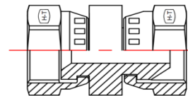
FJS-FBSPPS Straight
