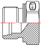
MM LIGHT SERIES TUBE PLUG (DIN2353 S)
