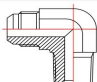
MJ-MBSPP 90° Elbow
