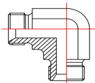
MBSP-MSPP 90° Elbow
