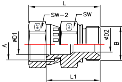
FJS-MM Straight
