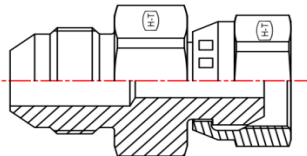
MJ-FBSPS Straight
