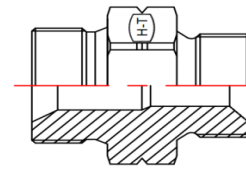
MBSP-MM Straight
