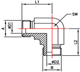
MBSPP-MBSPP 90° Elbow
