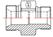
MBSP-MSPP Straight
