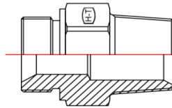
MBSP-MSPT Straight
